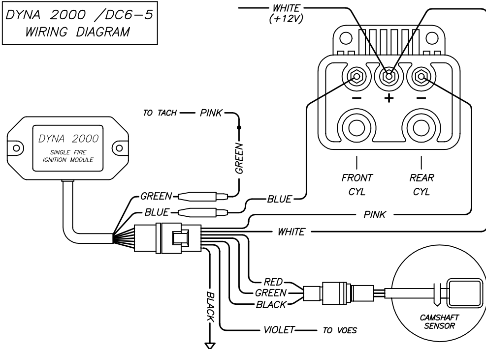
DYNA 2000i /DC6-5 WIRING DIAGRAM OUTPUTS REVERSED
